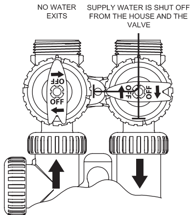
FIGURE 4 SHUT OFF MODE POSITION
