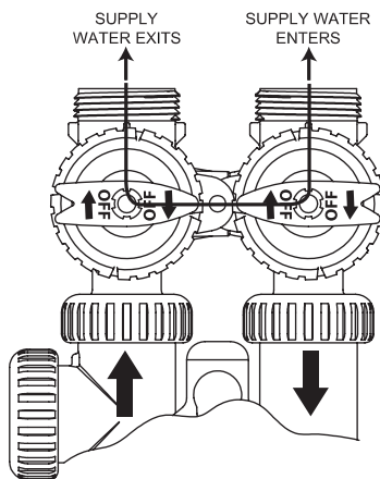
FIGURE 2 BYPASS OPERATION POSITION
